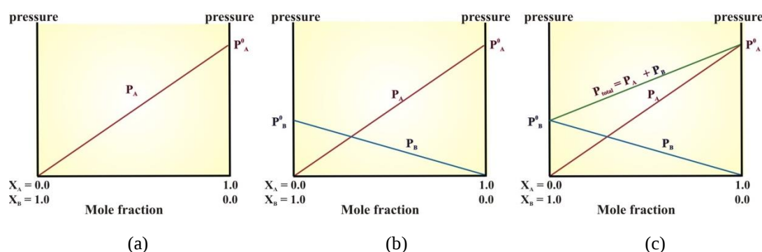
Figure 2.44 Vapour pressure – composition diagrams for an ideal mixture AB which obeys the Rault law at constant temperature. (a) Variation of vapour pressure of component A; (b) variation of vapour pressure of component B included and (c) variation in total vapour pressure of the mixture.
