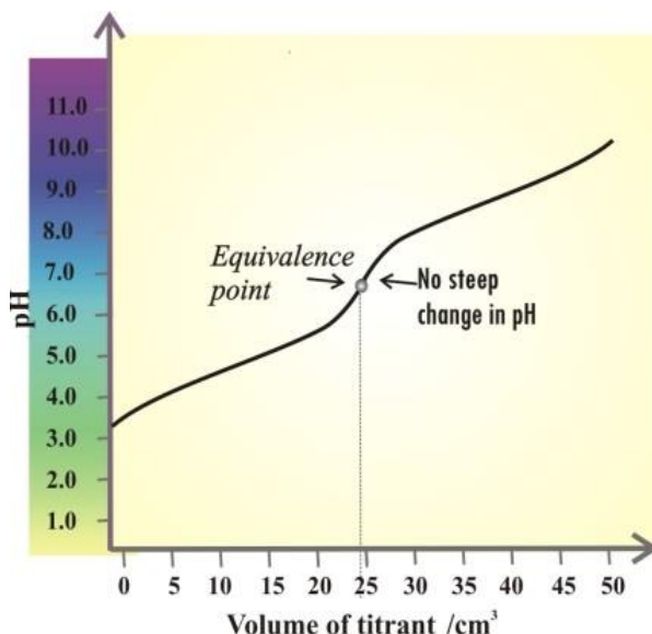
Figure 2.20 Titration curve for the titration of 25.00 cm 3 of 0.100 mol dm -3 CH 3 COOH with 0.100 mol dm -3 NH 3 . It is difficult to judge to location of the equivalence point as it depends on the relative strengths of the acid and the base. There is no steep change in pH in these types of systems.
